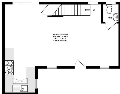
GROUND FLOOR CEILING HEIGHT 2.17 M 415 sq.ft. (38.6 sq.m.) approx.
